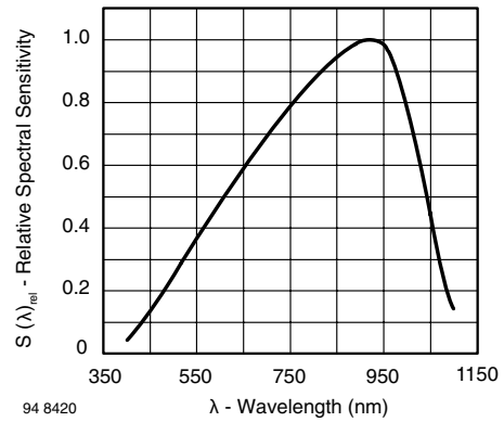
94 8420 Figure 7. Relative Spectral Sensitivity vs. Wavelength
