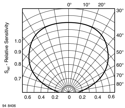
94 8406 Figure 8. Relative Radiant Sensitivity vs. Angular Displacement
