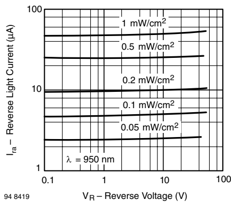
94 8419 Figure 5. Reverse Light Current vs. Reverse Voltage
