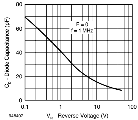
948407 Figure 6. Diode Capacitance vs. Reverse Voltage
